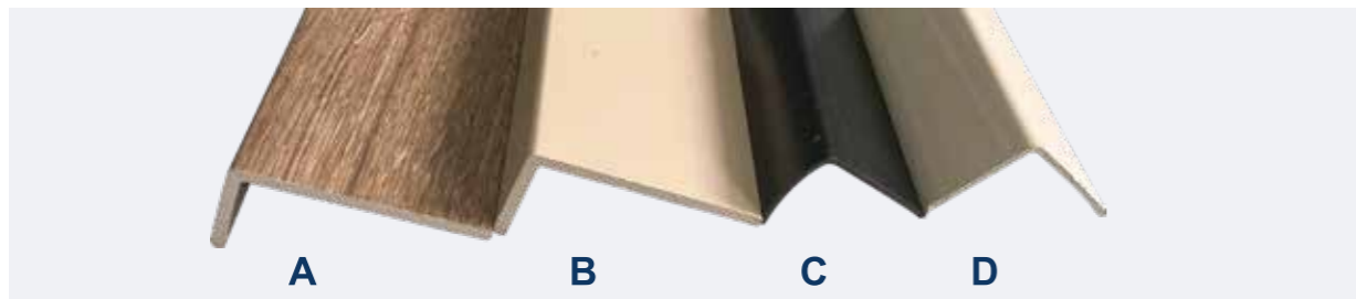
SPC Stairnose A:88*40*4.8mm B:88*41.7*4.4mm C:50*40*2mm D:51*50*2.5mm
