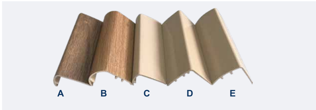
SPC Overlap Stairnose A:48*26*2.5mm B:54.5*40*2.1mm C:49.5*26*2.5mm D:51*48*2mm E:50*50*1.8mm
