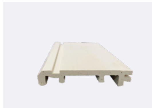
WPC Skirting Size: 2400*75*15mm
